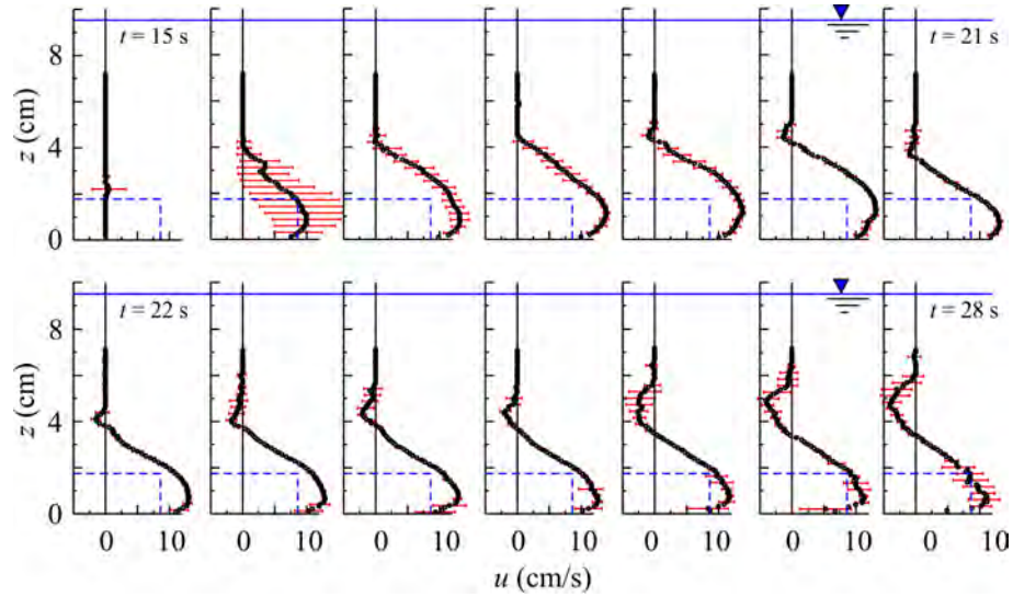
Figure 13: Velocity profiles for Exp. #34, \gamma = 0 (outflow section at the opposite end of the channel with respect to inflow section). For caption see Figure 12.
