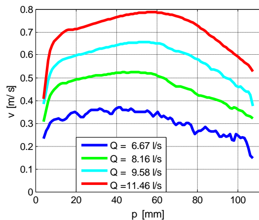
Fig. 7: Mean velocity profiles measured at various flow rates
