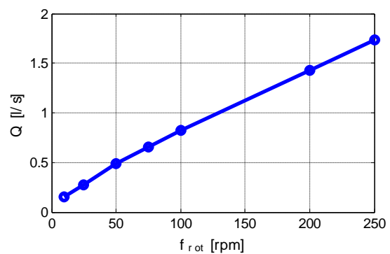
Fig. 5: Volume flow rate Q vs. rotation speed f_{rot} of the EM pump
