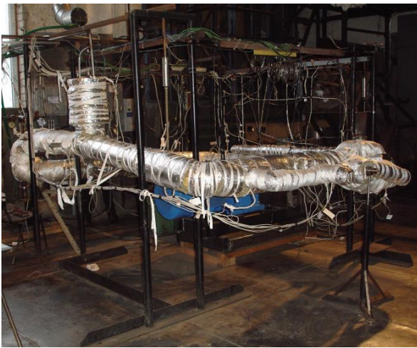
Fig. 6: META:LIC loop with measurement locations
