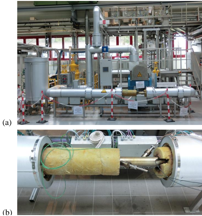
Fig. 2: LIMMCAST facility: (a) general view, (b) test section
