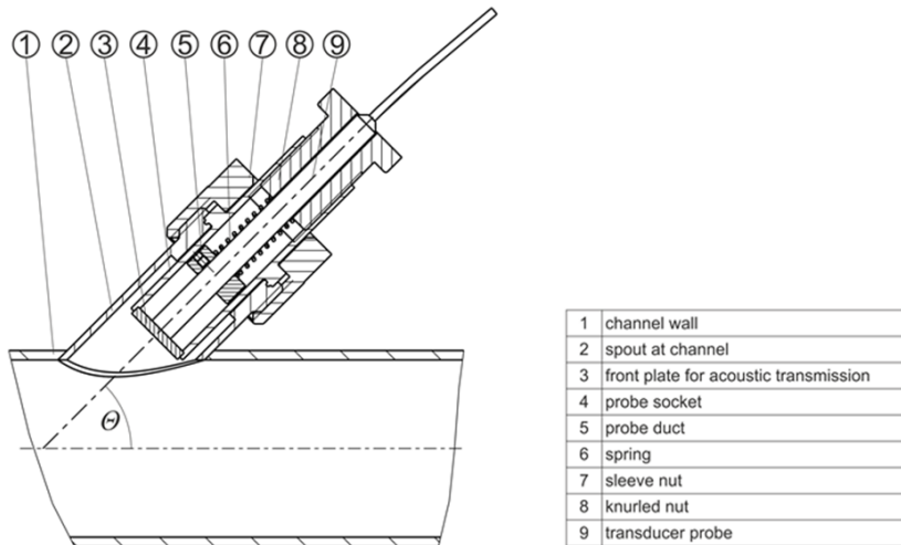
Fig. 1: Probe socket design
