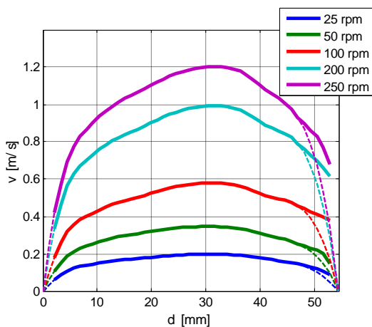
Fig. 4: Mean flow velocity for various rotation speeds of the EM pump (velocity values are corrected with respect to the Doppler angle)
